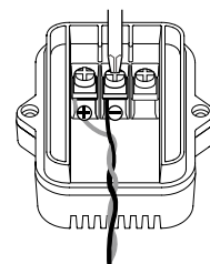
Thermocouple sensor
