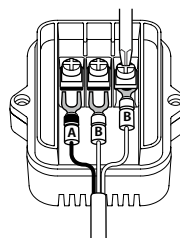
Pt sensor
