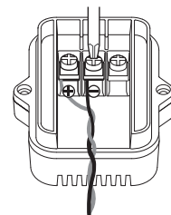
Thermocouple sensor
